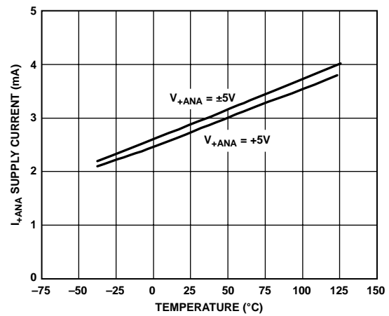
Figure 14. I_{+ANA} Supply Current/Comparator vs. Temperature
