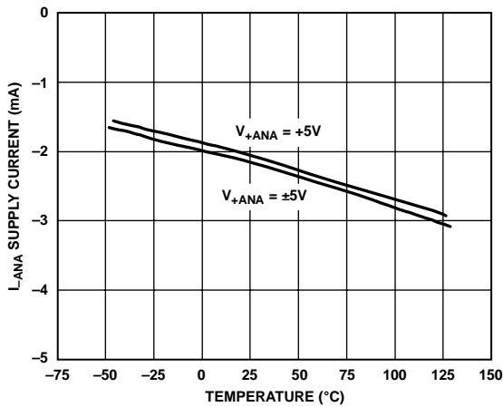
Figure 15. I_{-ANA} Supply Current/Comparator vs. Temperature
