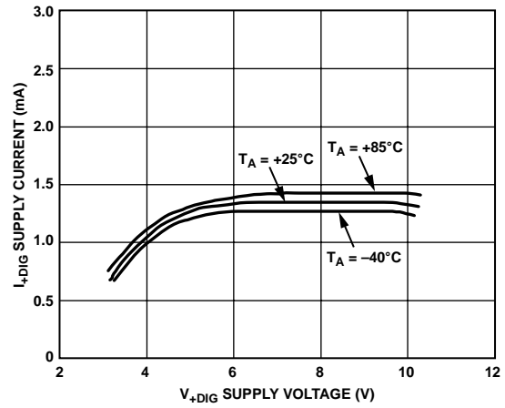
Figure 13. I_{+DIG} Supply Current/Comparator vs. V_{+DIG} Supply Voltage
